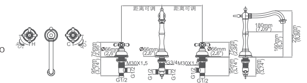
Model No:C-31 Lavatory Faucet
