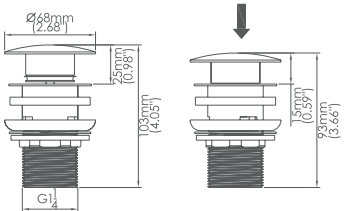
Model No:POP-03 pop-up waste for washbasin
