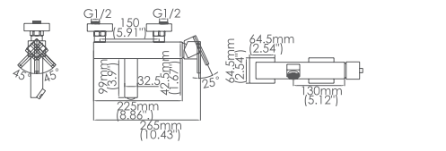
Model No:H-38 Bathtub Shower
