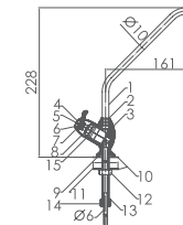
Model No:JD-16A Filter faucet
