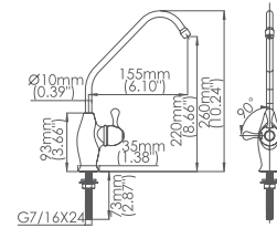
Model No:F-1B Filter faucet
