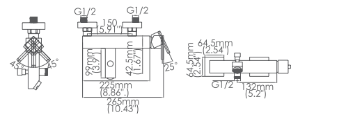
Model No:H-30 Bathtub Shower
