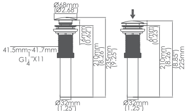
Model No:POP-03 pop-up waste for washbasin
