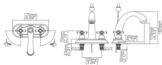
Model No:C-21 Lavatory Faucet
