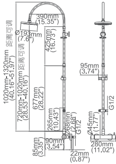
Model No:G-29C Thermostatic Shower
