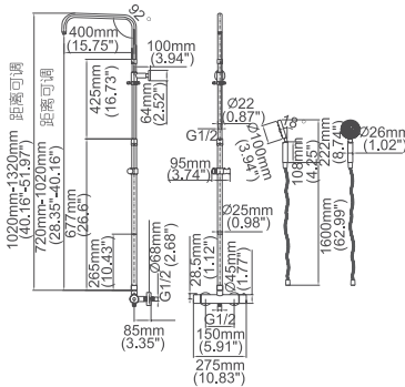
Model No:G-36B Thermostatic Shower
