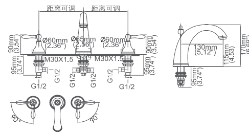
Model No:C-19 Lavatory Faucet
