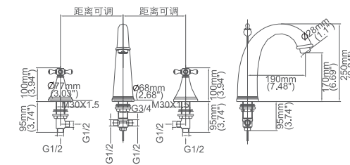
Model No:C-17 Bathtub Shower
