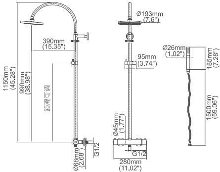
Model No:G-36A Thermostatic Shower
