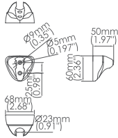
Model No:B-96 Hand Shower Holder
