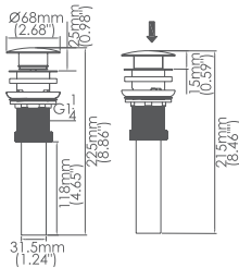
Model No:POP-01 pop-up waste for washbasin
