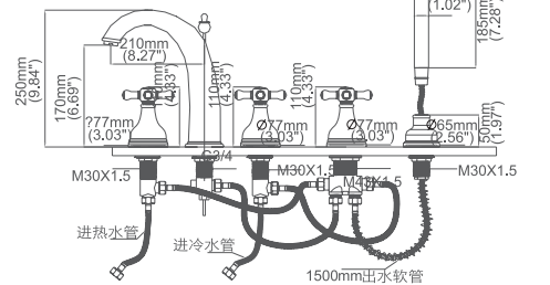
Model No:C-30 Bathtub Shower
