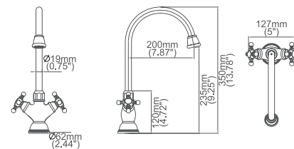
Model No:C-20 Lavatory Faucet
