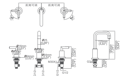
Model No:C-38-HYD Lavatory Faucet
