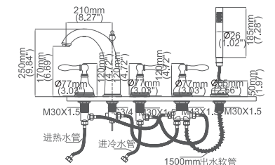
Model No:C-32 Bathtub Shower
