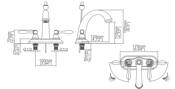
Model No:C-22 Lavatory Faucet
