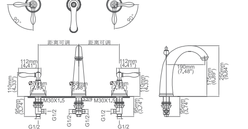
Model No:H-38 Bathtub Shower
