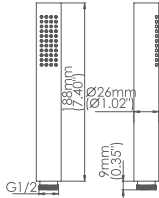
Model No:B-77B Hand Shower
